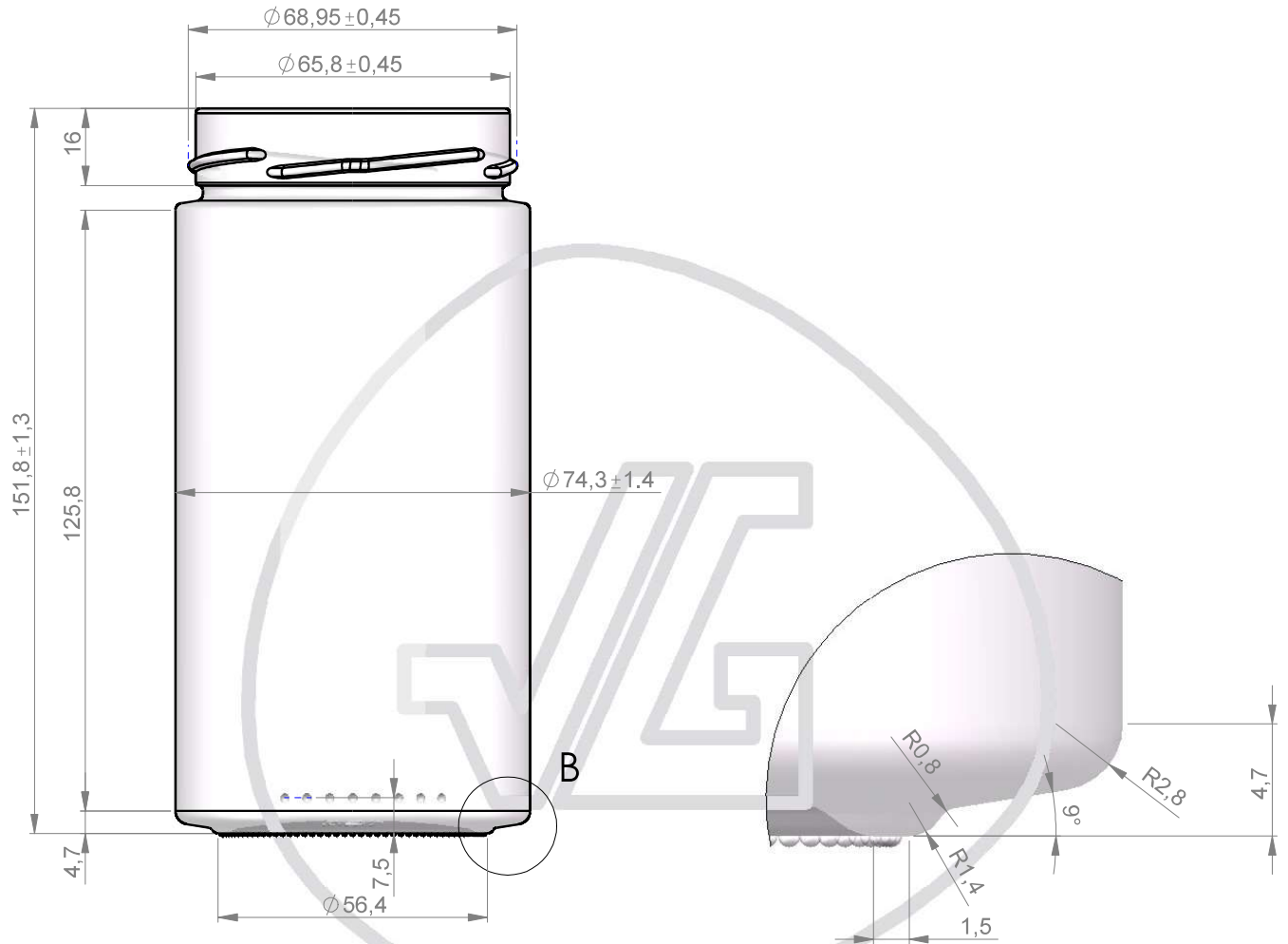
DETAIL B SCALE 5 : 1
