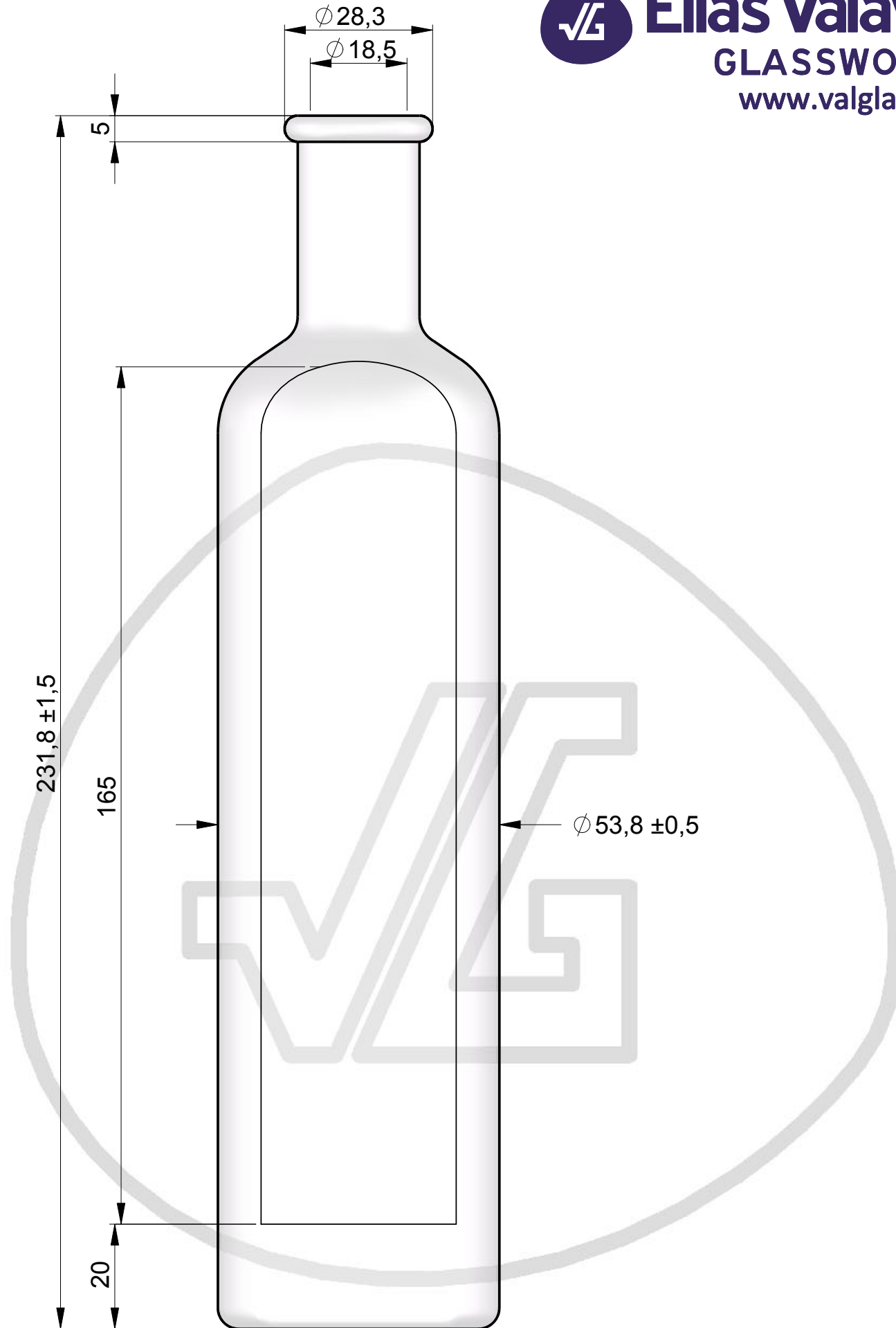
FRONT VIEW
