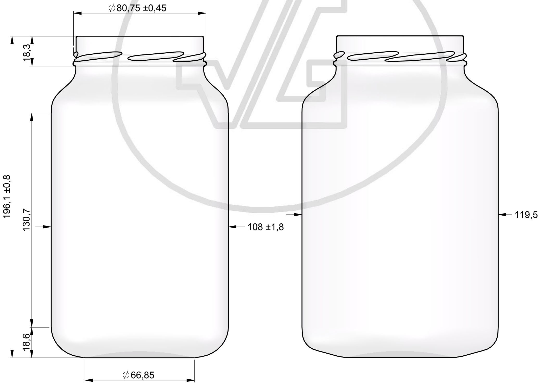
FRONT VIEW
