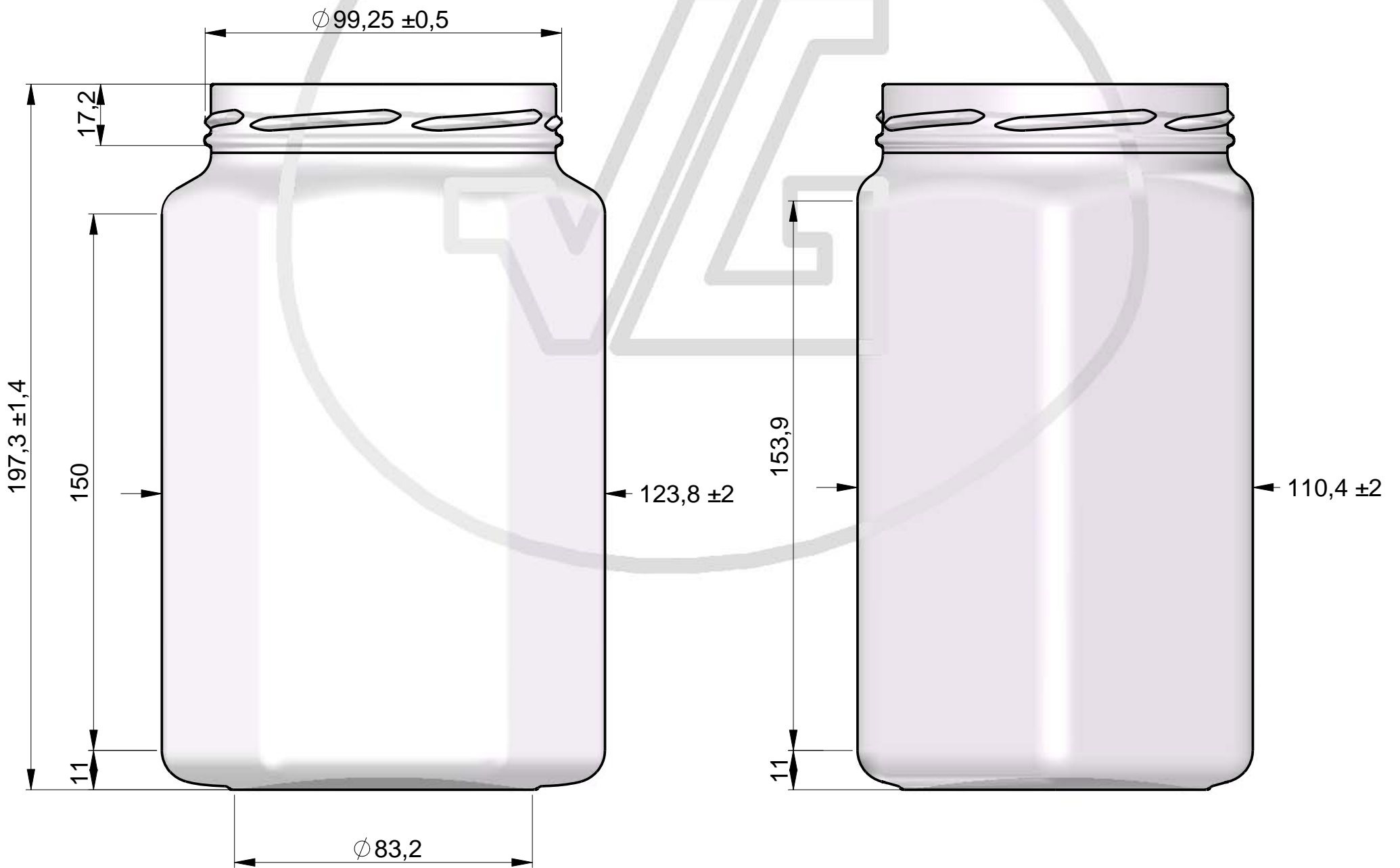
SIDE VIEW
