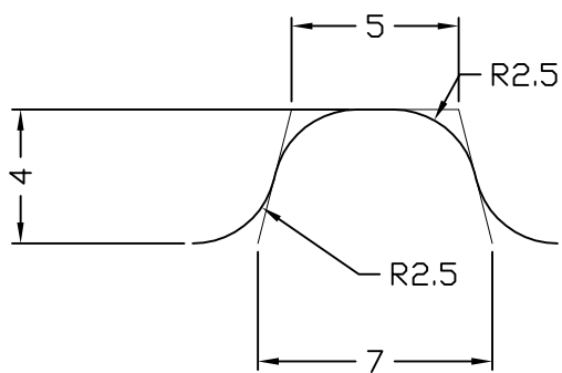
Guide Detail (Scale 4:1)
