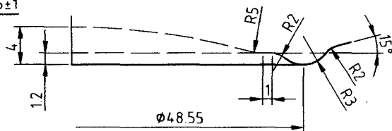
DETAIL A SCALE 2:1
